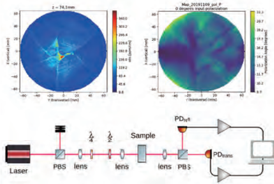
Top: results of ultra-precise measurements to relate the absorption coefficient (in ppm/cm) of Sapphire mirror-substrates with inherent birefringence. Bottom: principal setup for birefringence measurements
